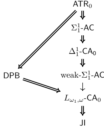
FIGURE 1. DPB, ATR_0 , and some theories of hyperarithmetic analysis. The new results are those concerning DPB. A double arrow indicates a strict implication.
